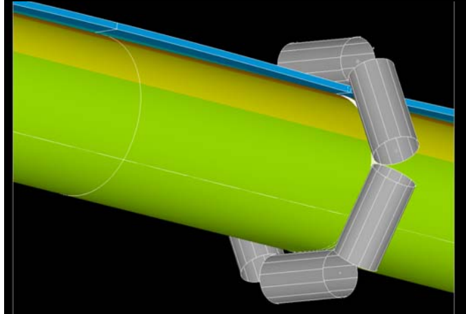
Figure 5. Comparison of a 400mm ST1250 Confine pipe belt with a FEA model of the same belt.
