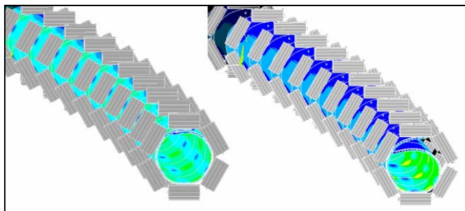
Figure 6. FEA simulation of Confine (left) and conventional (right) pipe belt during horizontal curves.
