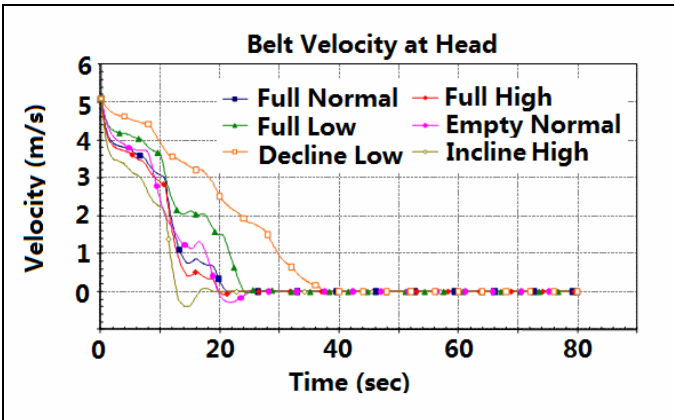
Figure 10. Dynamic analysis of pipe conveyor starting.
