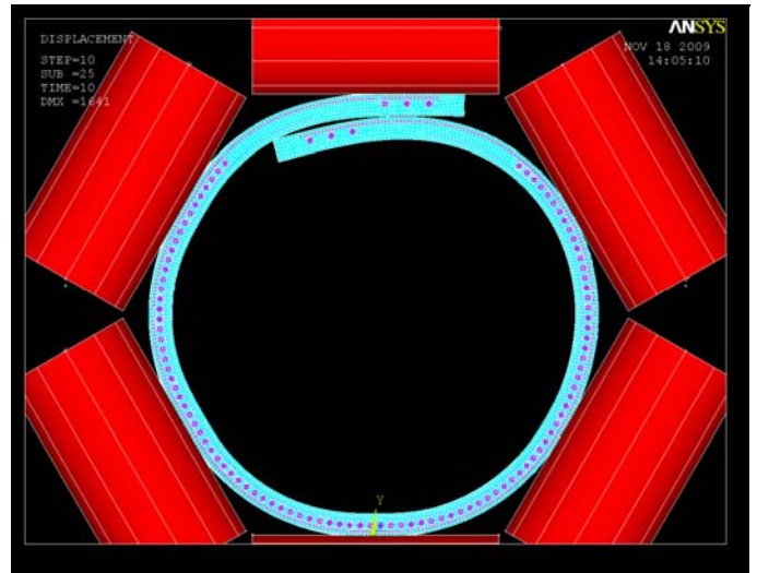
Figure 4. FEA of 500mm ST4000 Confine Pipe belt.
